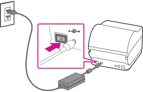
Power Cable
